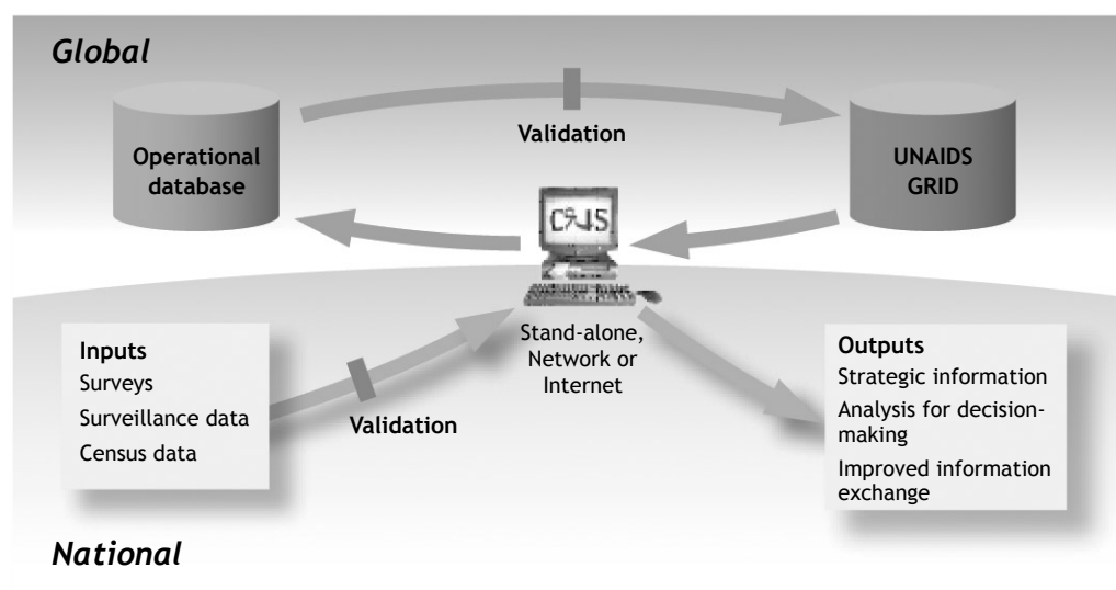
Figure 1. Data flows
